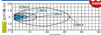
AB3023/3021 50Hz
