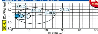
AB273/271/271P 50Hz
