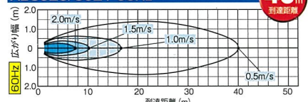
AB3023/3021 60Hz
